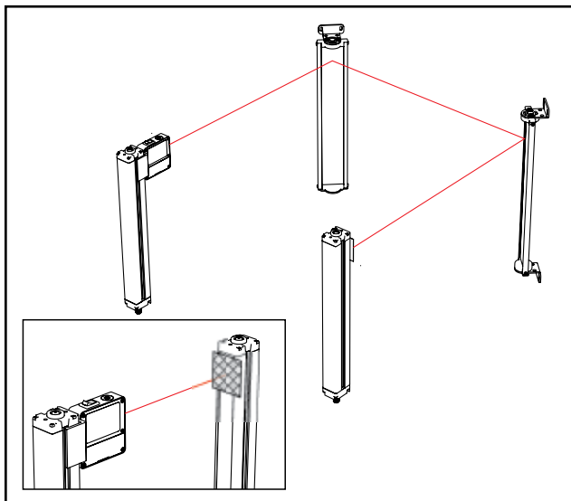
Figure 3-13. Optical alignment using the LAT-1
