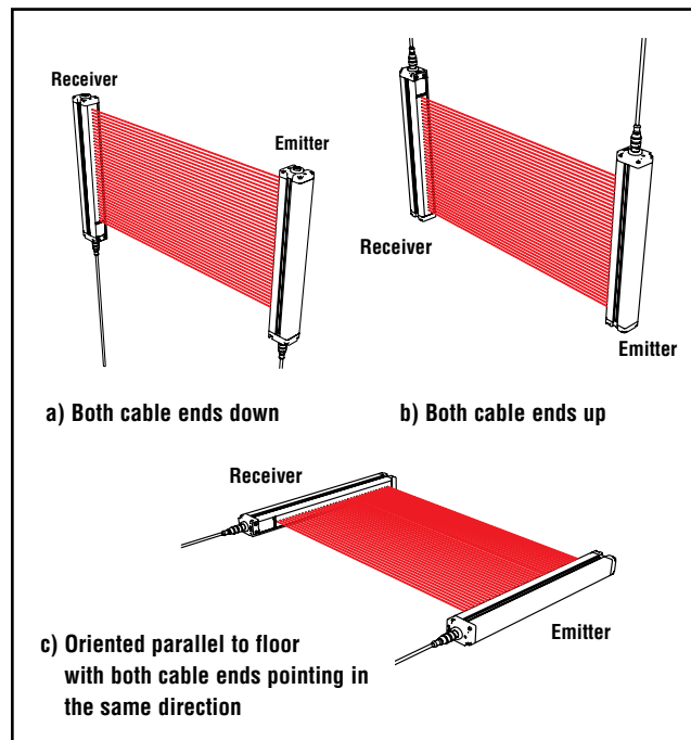
Figure 3-5. Examples of correct emitter / receiver orientation
