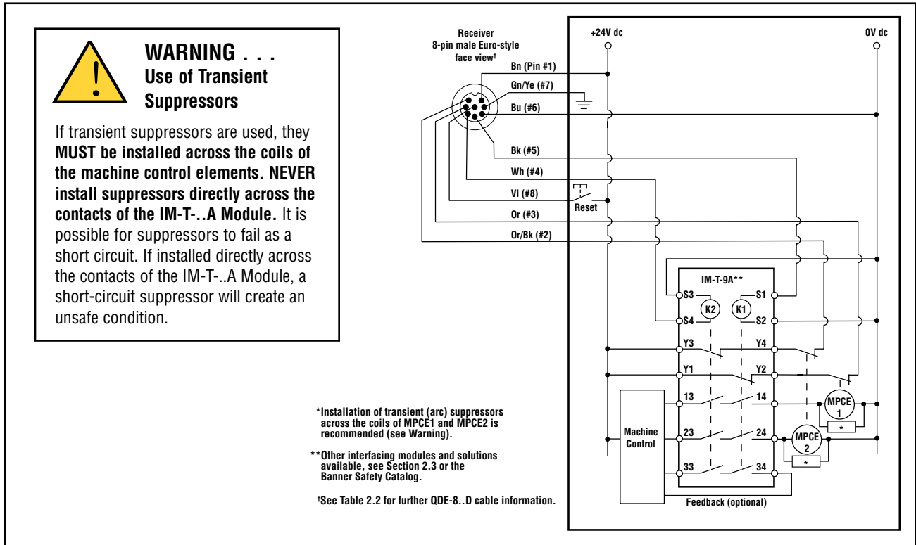
Figure 3-19. Generic hookup – interface module (2-channel EDM, manual reset)
