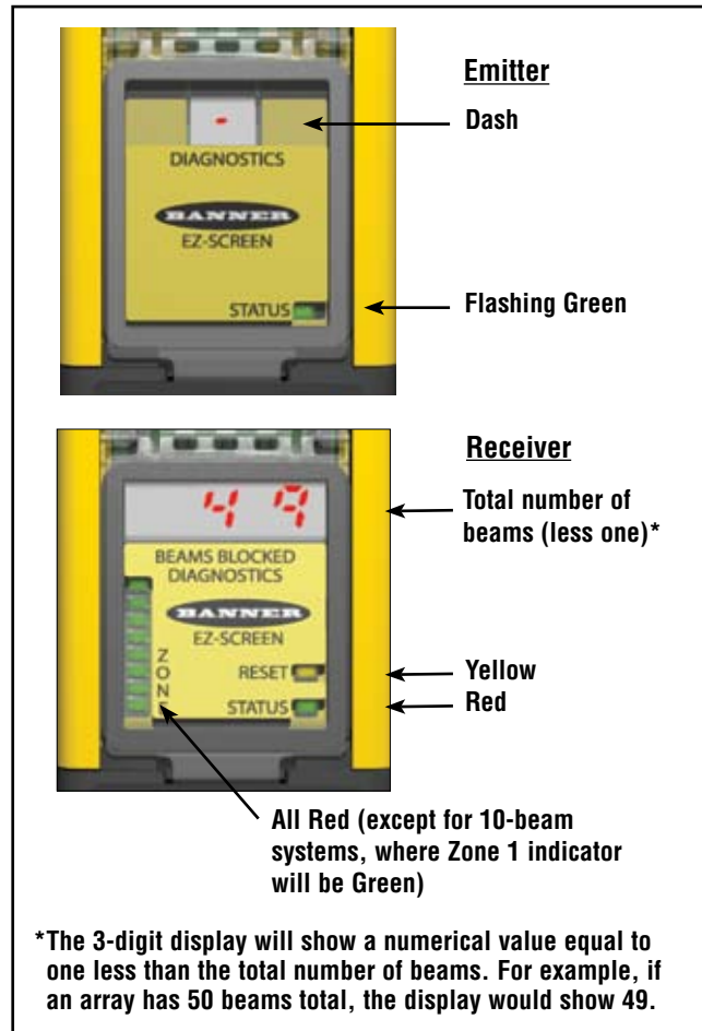
Figure 5-1. TEST mode status indicators
