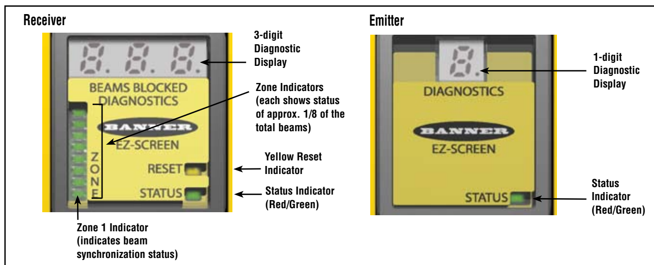
Figure 1-3. EZ-SCREEN emitter and receiver status indicators
