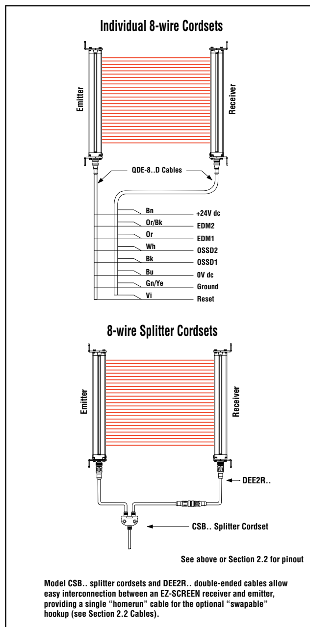
Figure 3-16. Emitters and receivers interchange easily when 8-pin connectors are used for both (optional hookup)
