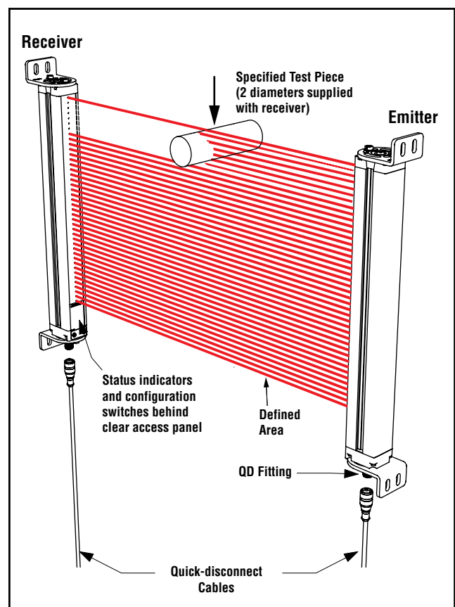
Figure 1-1. Banner EZ-SCREEN High-Resolution System: emitter, receiver, and two interconnecting cables
