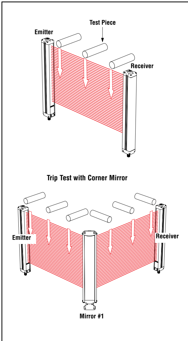
Figure 3-15. EZ-SCREEN trip test
