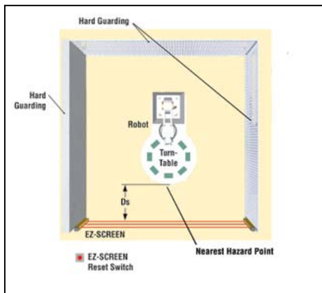
Figure 3-1. Separation distance and hard guarding
