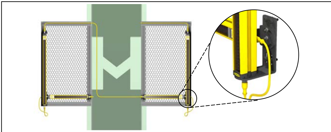
Figure 7-1. Multiple cascaded light screens used to guard two areas of one machine (power press cross-section, receivers only shown using EZA-MBK-21 “L” mounting bracket system)
