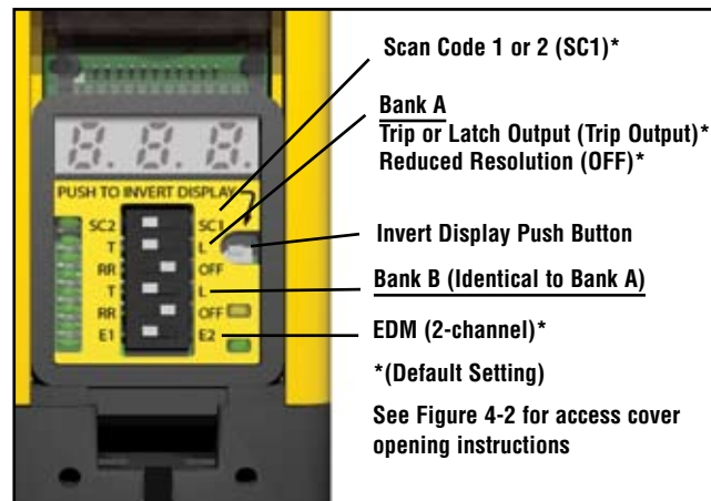
Figure 4-1. EZ-SCREEN configuration switches (receiver shown)
