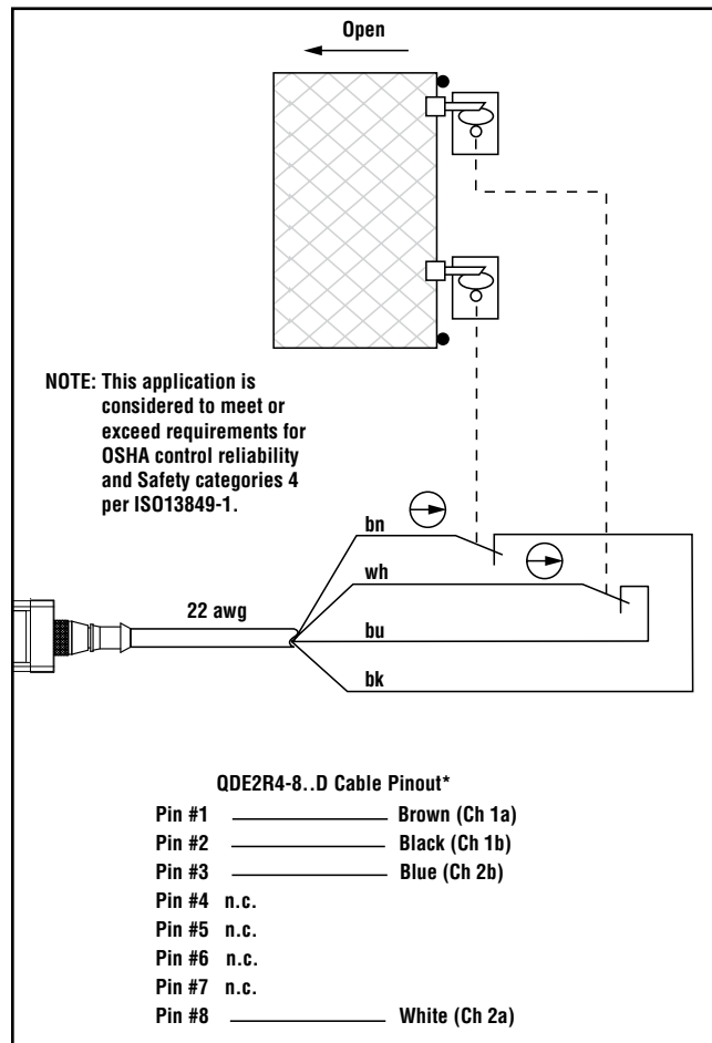
Figure 7-9. Monitoring two positive-opening safety switches
