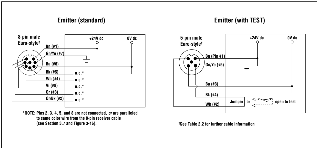
Figure 3-17. Emitter; generic hookup
