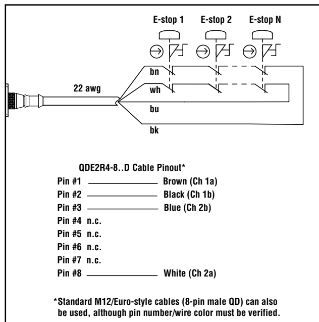
Figure 7-8. Hookup of E-stop buttons to the last receiver in the cascade
